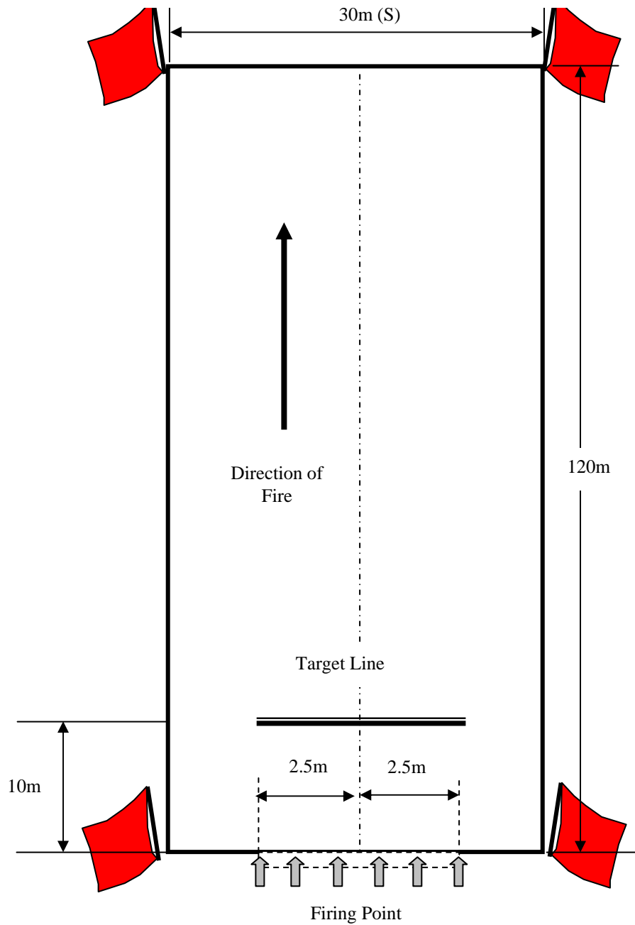
Figure 26-2. Air Rifle Range, Layout, Including Range Danger Area (RDA).
